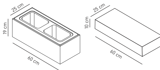
PUSTAK 60/25/19 DASZEK NISKI 60/25/10
